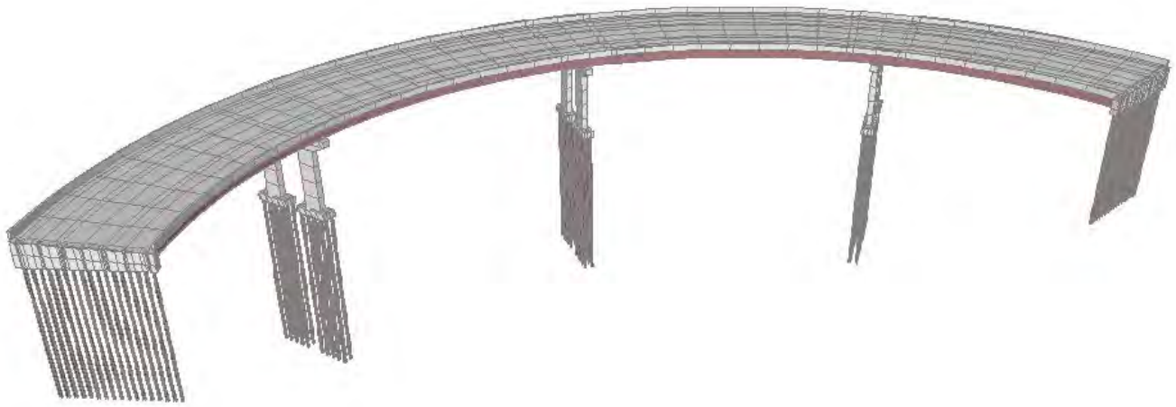
Figure 1.7 - SAP2000® Finite Element Model of the I-480 Bridge in Nebraska [8]
