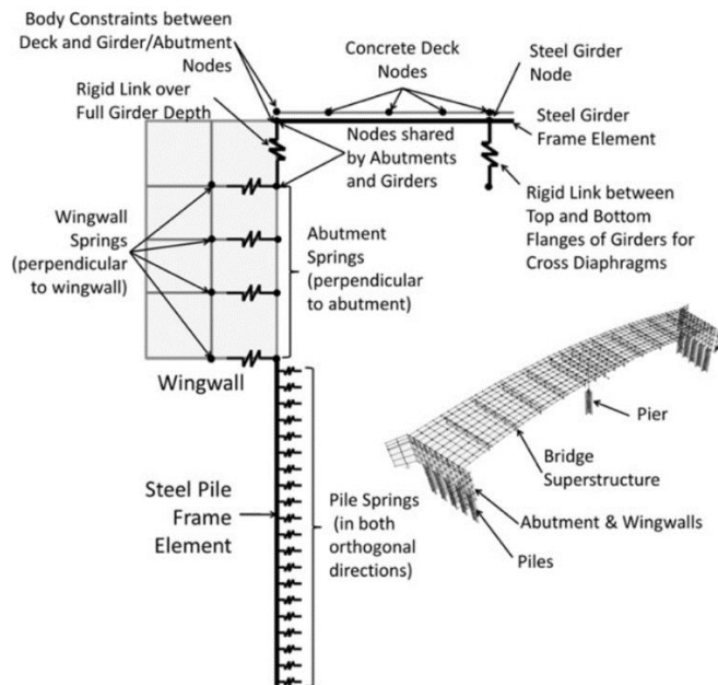
Figure 1.4 - Structural Component Mesh and Connectivity of the Stockbridge Bridge [5]
