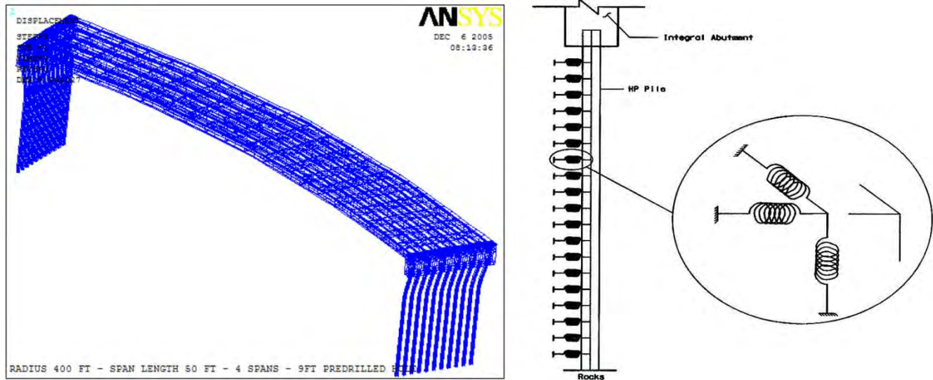
Figure 1.8 - ANSYS® Model and Pile Support Representation for Integral Abutment Bridge Model [1]
