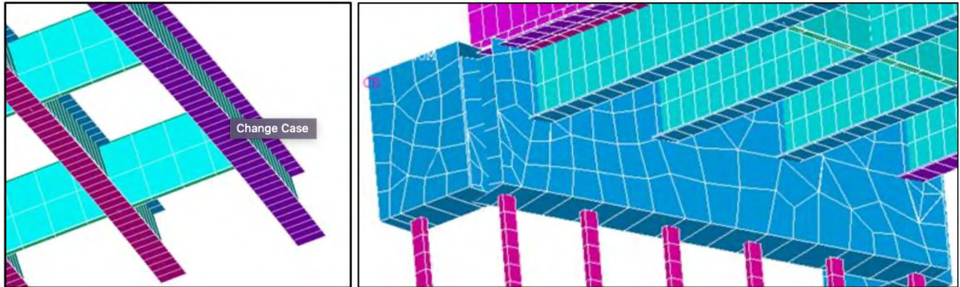
Figure 1.6 - ANSYS® Model of Bridge 309, Illustration of Structural Component Mesh and Connectivity [7]
