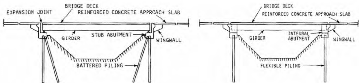
Figure 1.1 - Schematic of a Jointed Bridge (Left) and an Integral Abutment Bridge (Right) [2]
