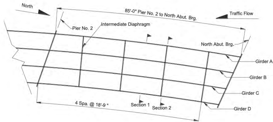
Figure 1.5 - Plan View of Bridge 309 Instrumentation Sections [7]
